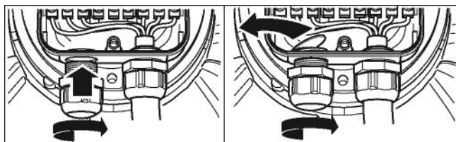
III. 4: Screwed cable gland opening
