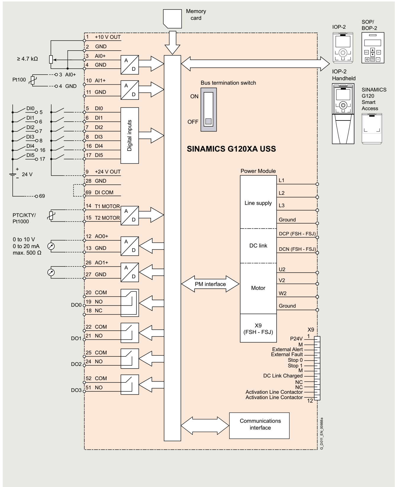
SINAMICS G120XA, USS version, connection diagram
