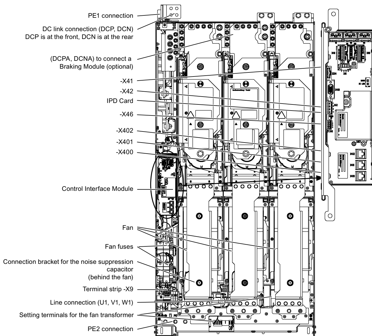
Figure 3-12 Smart Line Module, frame size JX
