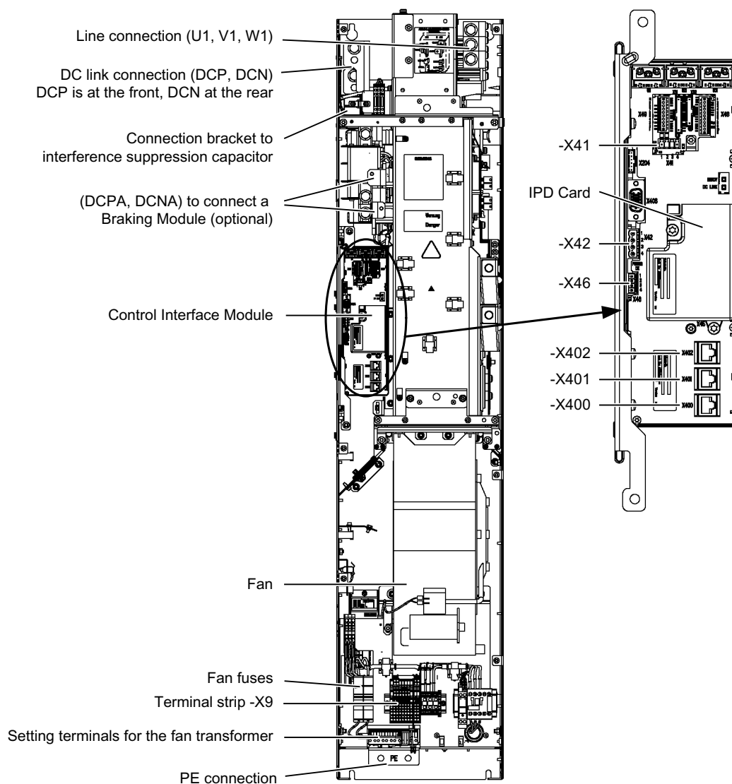
Figure 3-10 Smart Line Module, frame size GX
