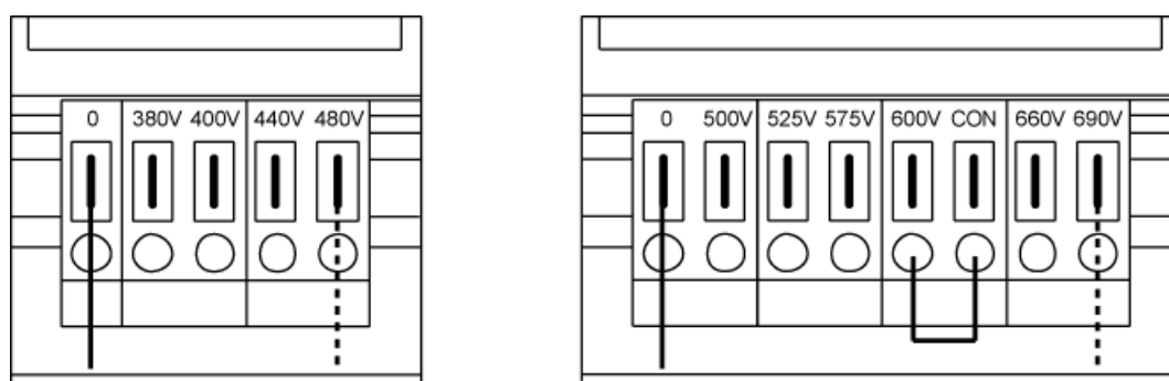
Figure 3-31 Setting terminals for the fan transformers (380 V – 480 V 3 AC / 500 V – 690 V 3 AC)
