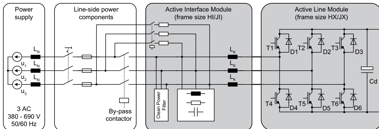
Figure 3-21 Overview of Active Infeed (frame sizes HI/HX and JI/JX)
