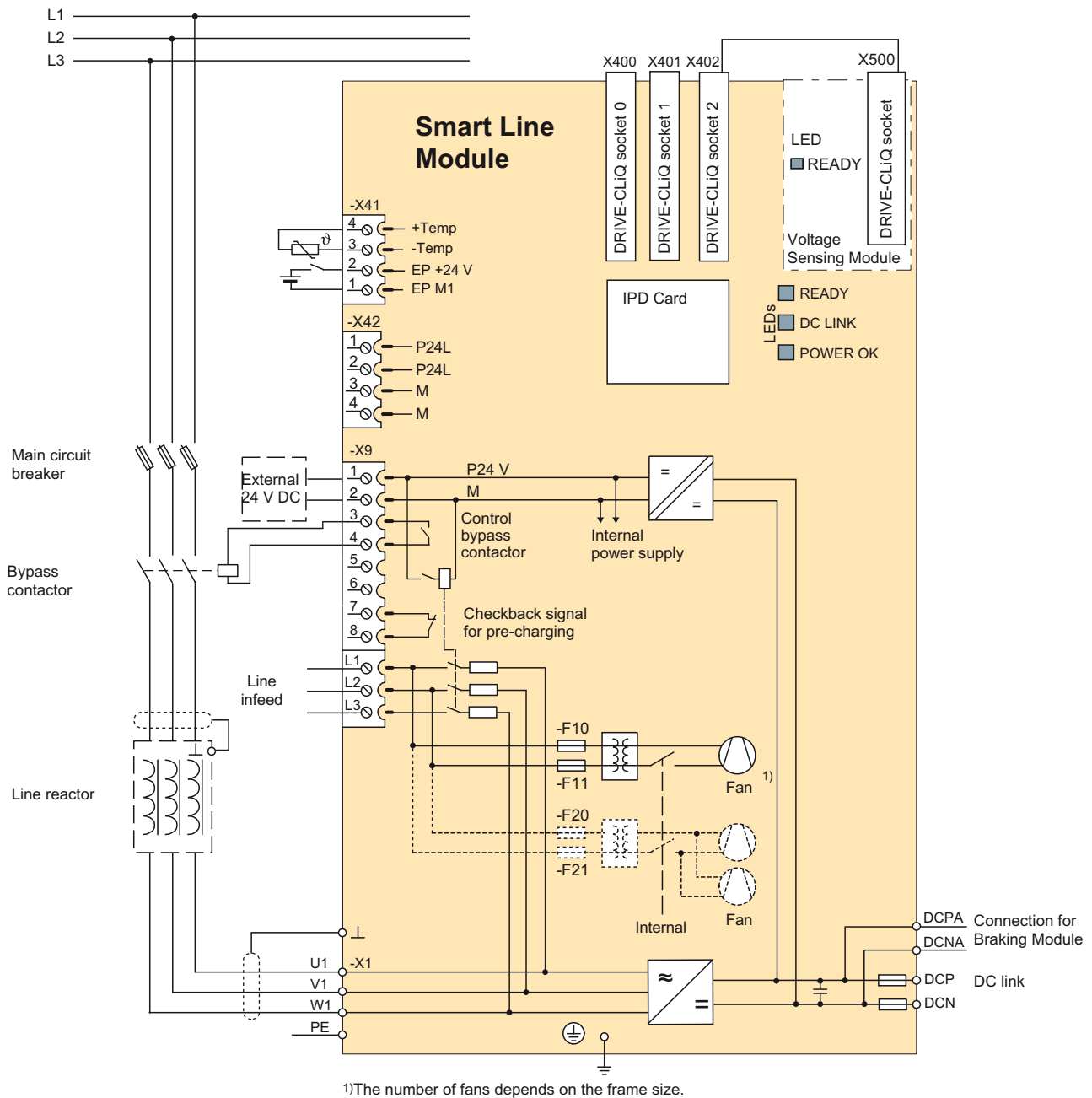
Figure 3-13 Smart Line Module wiring diagram
