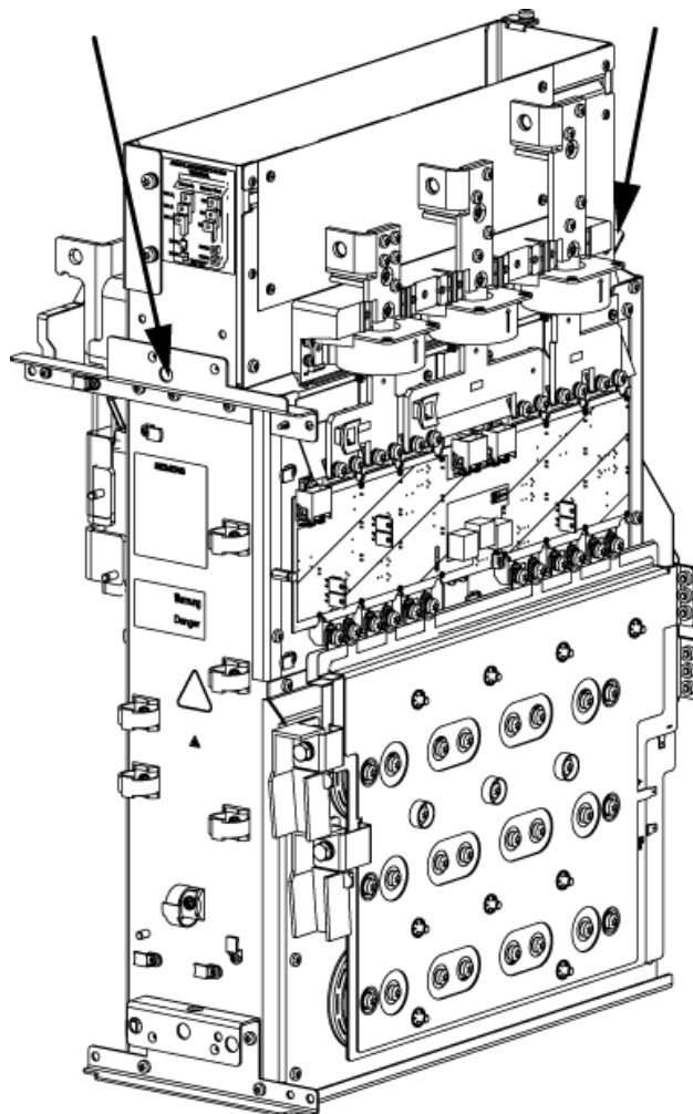
Figure 8-2 Crane lifting lugs on power block frame size FX, GX, FB
