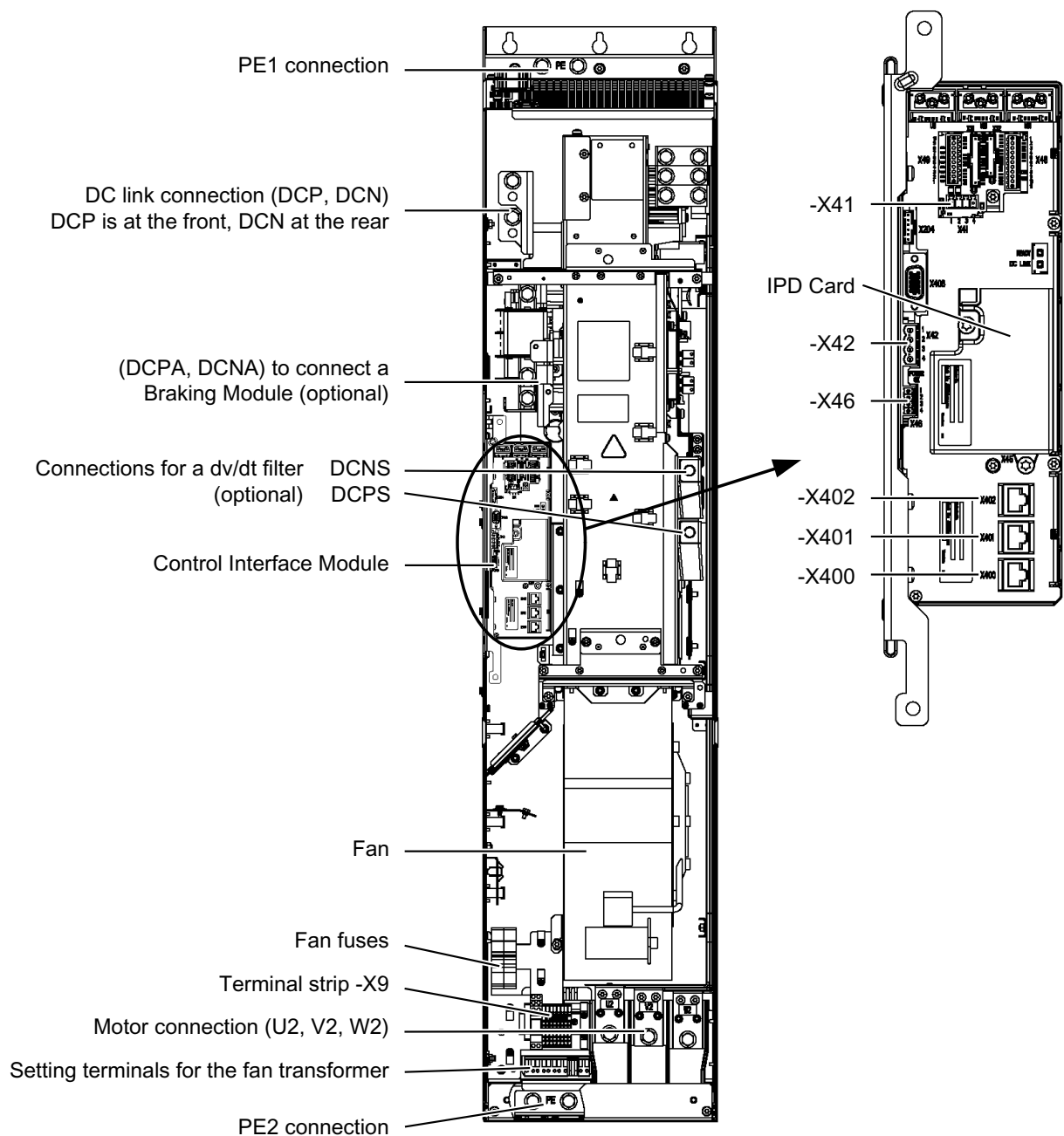
Figure 4-2 Motor Module, frame size GX
