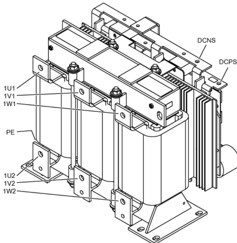
Figure 6-15 Interface overview for dv/dt filter compact plus Voltage Peak Limiter, Type 3
