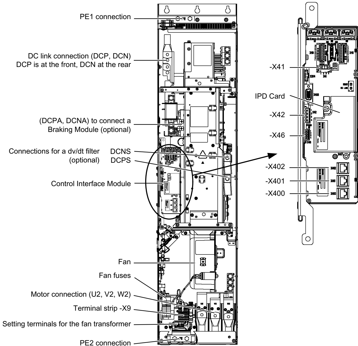
Figure 4-1 Motor Module, frame size FX
