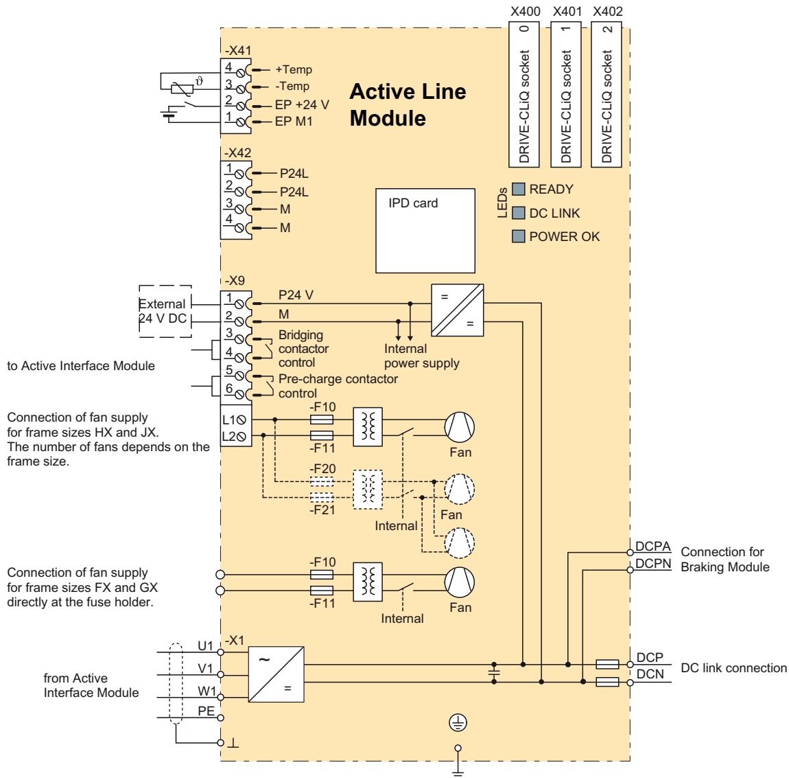
Figure 3-26 Active Line Module wiring diagram
