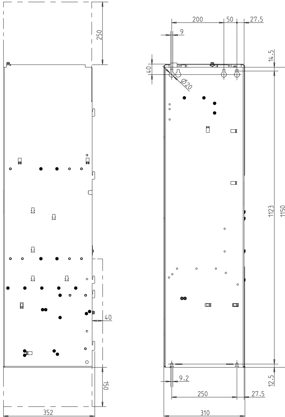
Figure 3-4 Dimension drawing, Basic Line Module, frame sizes FB, side view, front view
