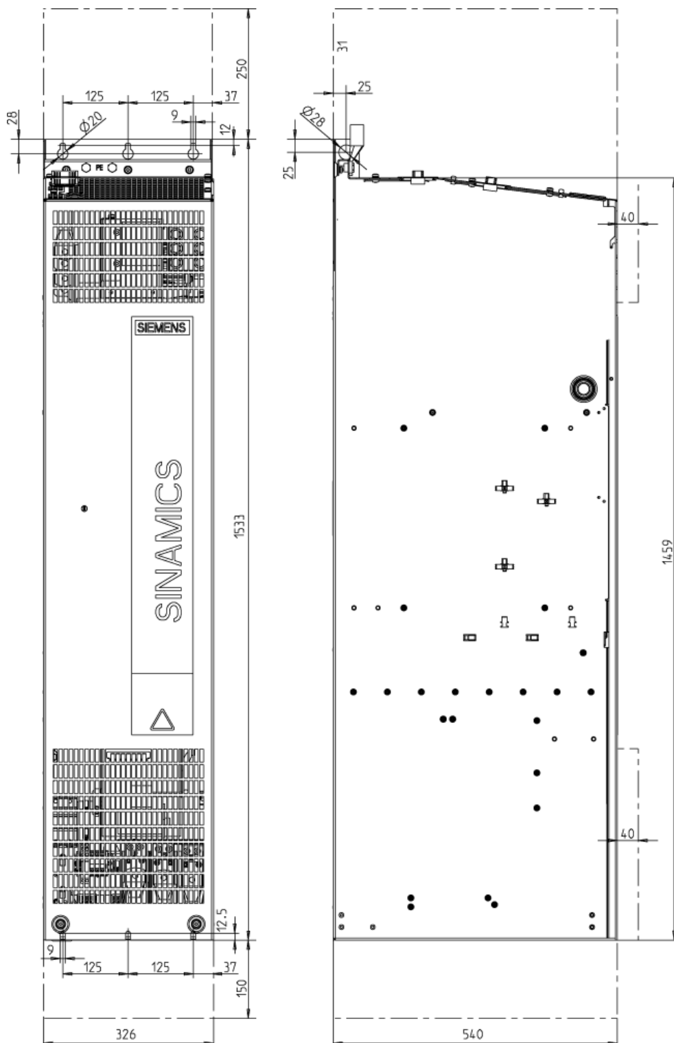
Figure 3-28 Dimension drawing Active Line Module, frame size GX Front view, side view
