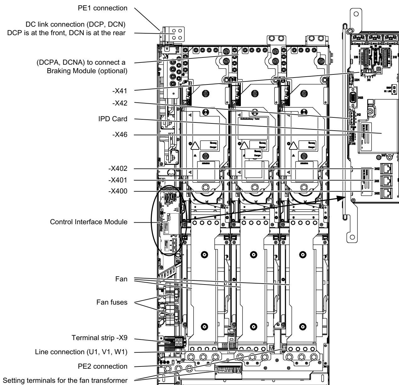
Figure 3-25 Active Line Module, frame size JX
