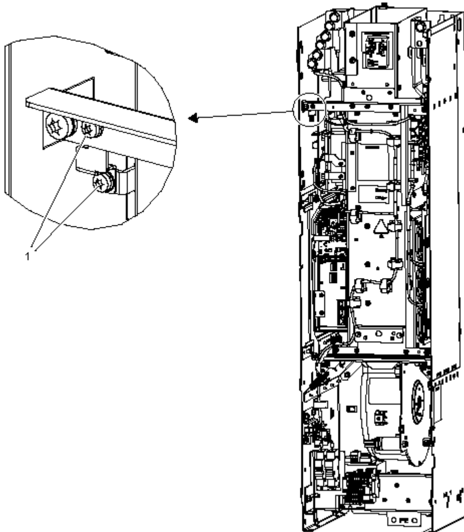
Figure 3-6 Removing the connection bracket to the noise suppression capacitor (example: frame size FB)
