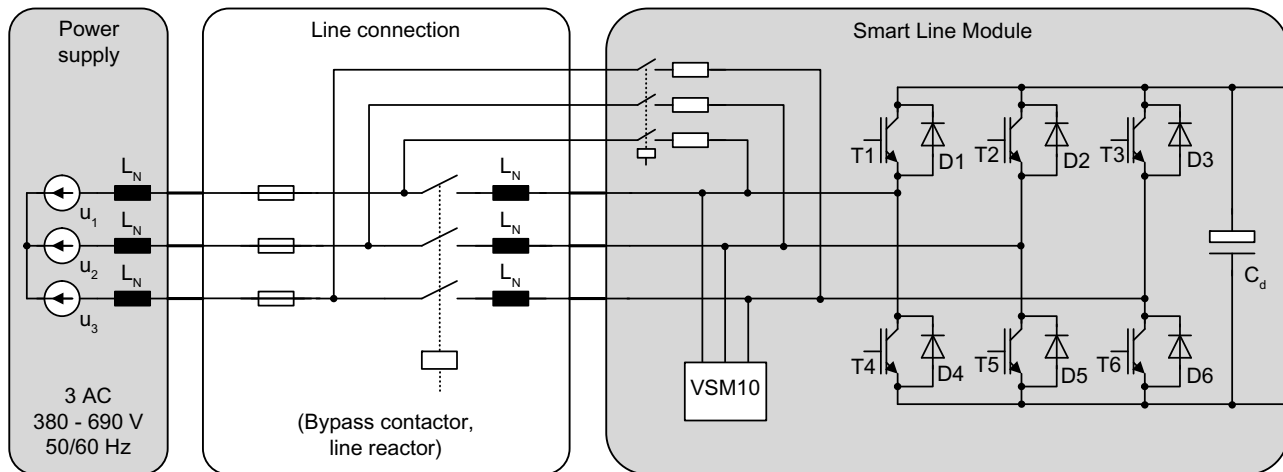
Figure 3-9 Overview of Smart Infeed
