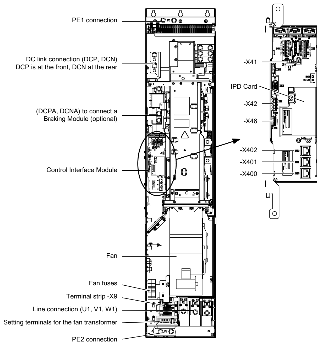
Figure 3-23 Active Line Module, frame size GX
