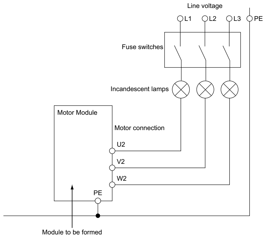
Figure 8-29 Forming circuit for Motor Modules
