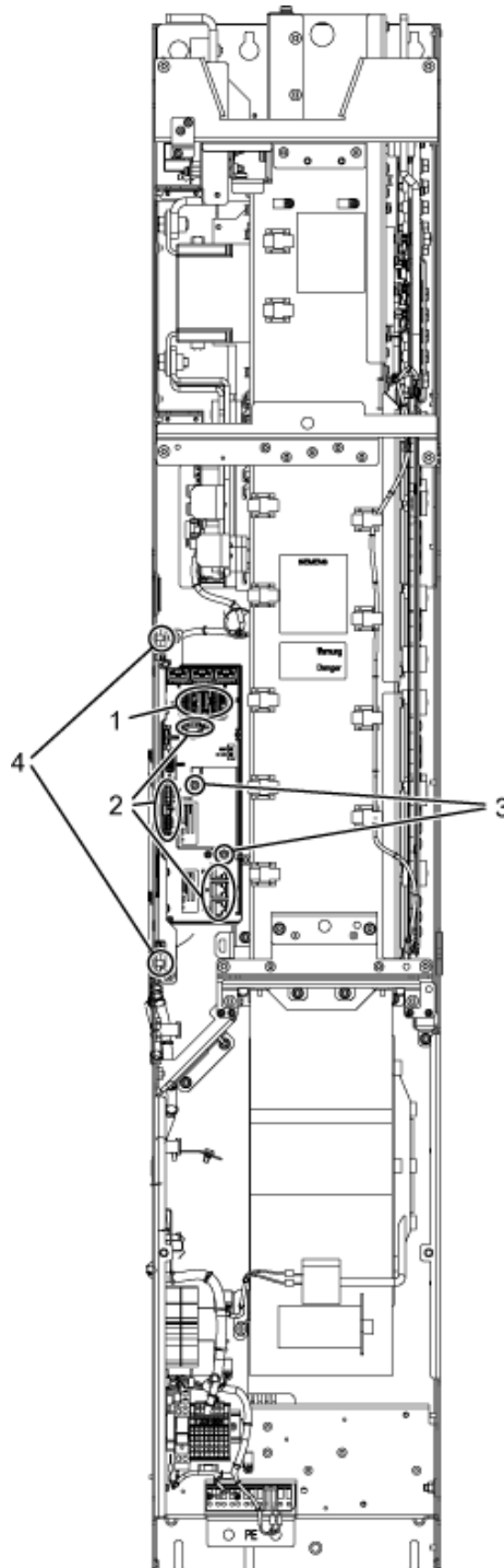
Figure 8-17 Replacing the Control Interface Module, Basic Line Module, frame size GB
