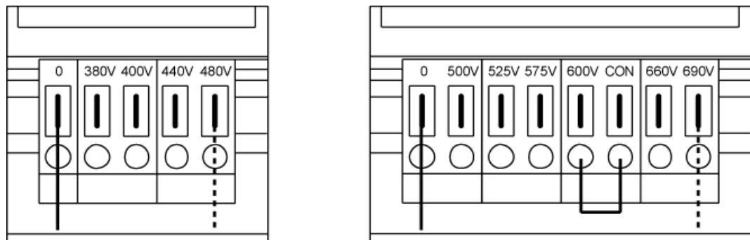
Figure 4-10 Setting terminals for the fan transformers (380 V – 480 V 3 AC / 500 V – 690 V 3 AC)
