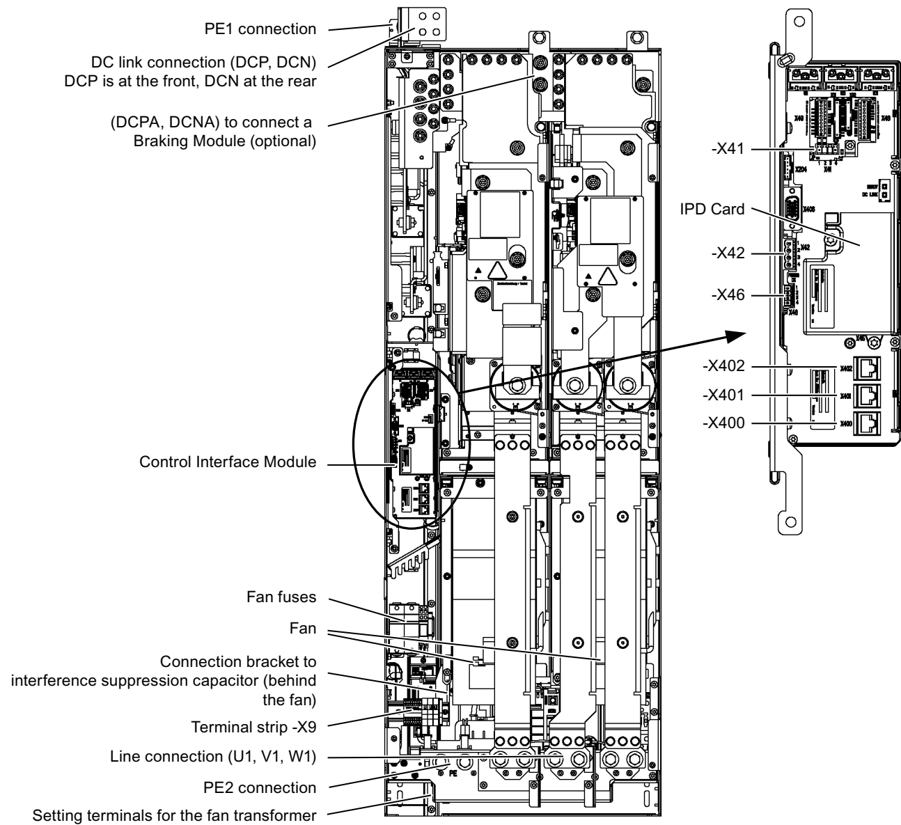
Figure 3-11 Smart Line Module, frame size HX
