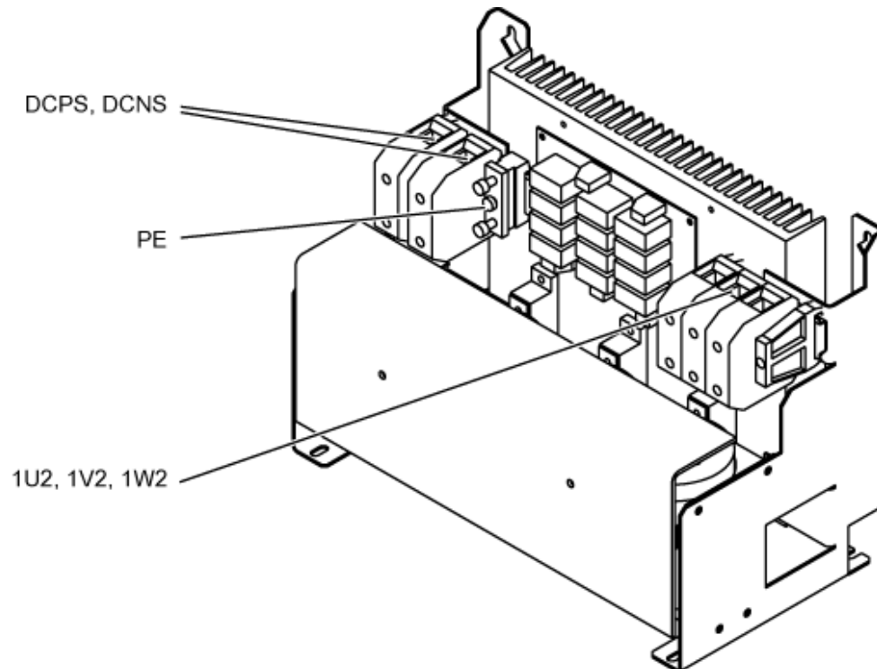
Figure 6-5 Interface overview, voltage peak limiter, type 2
