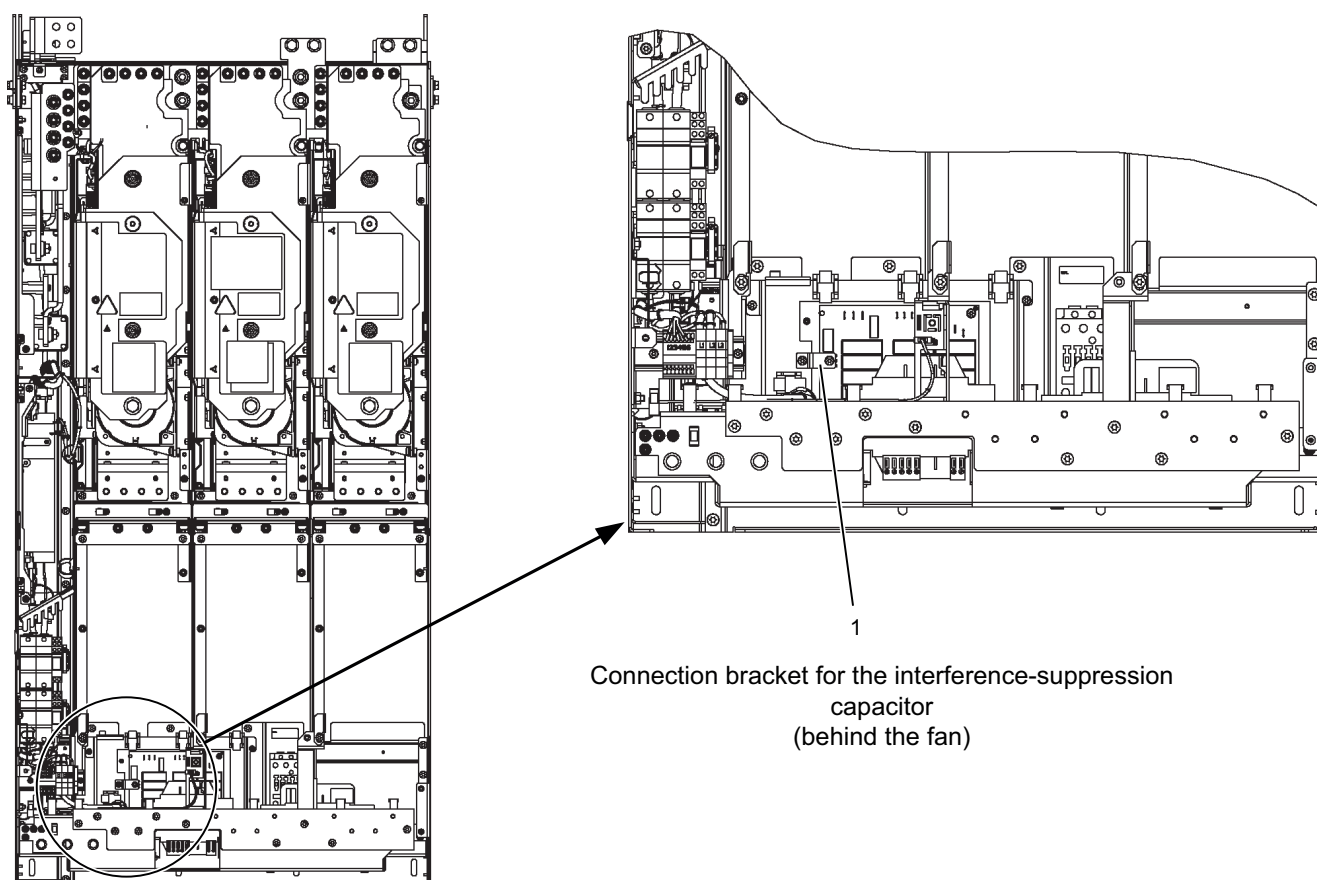
Figure 3-17 Removing the connection bracket to the noise suppression capacitor (example: Frame size JX)
