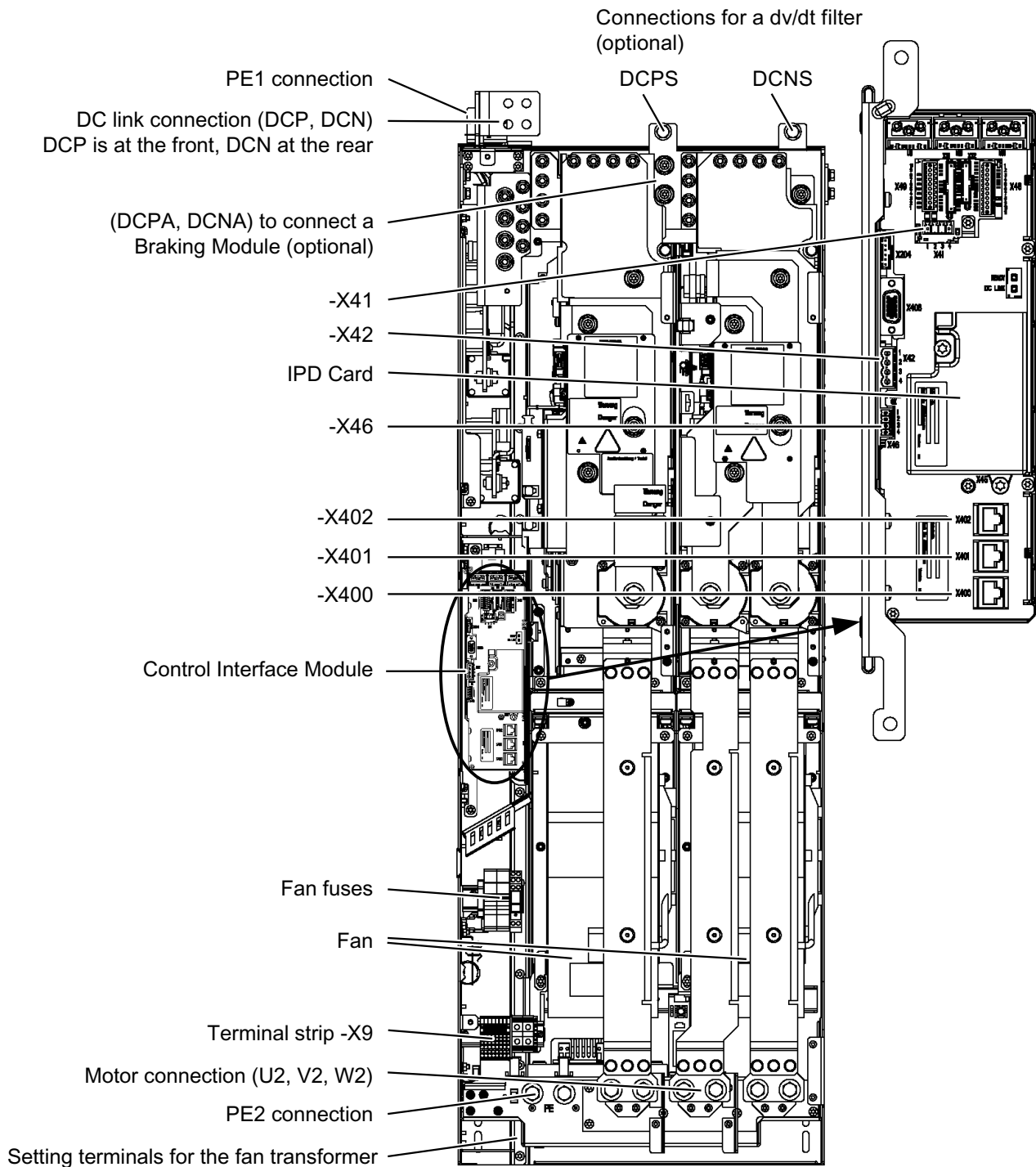
Figure 4-3 Motor Module, frame size HX
