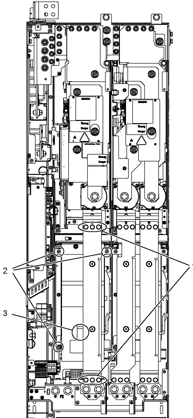
Figure 8-19 Replacing the fan, Smart Line Module, Active Line Module and Motor Module, frame size HX - left power block
