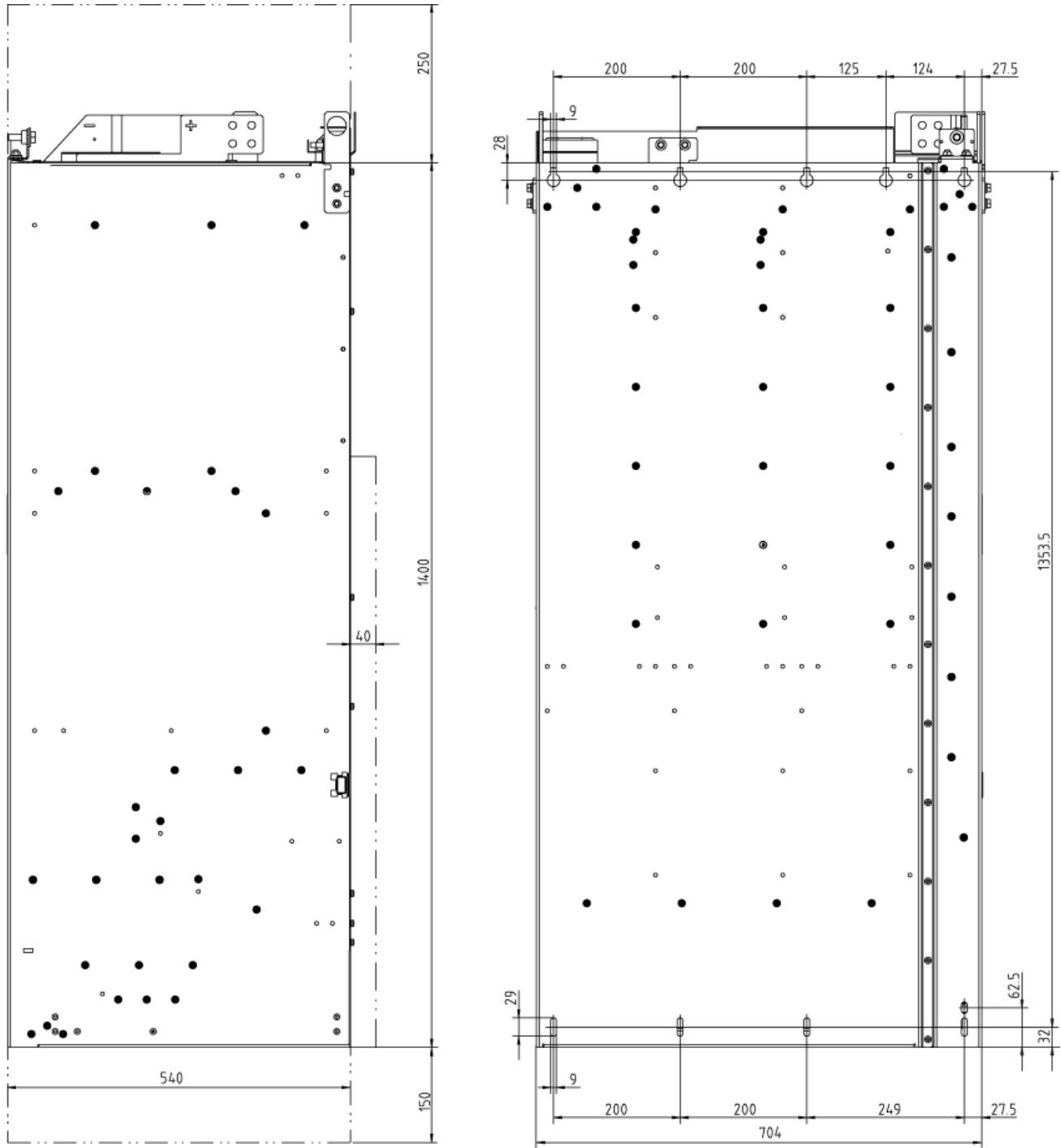
Figure 3-16 Dimension drawing Smart Line Module, frame size JX Side view, rear view
