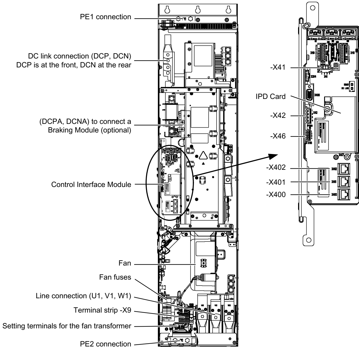
Figure 3-22 Active Line Module, frame size FX
