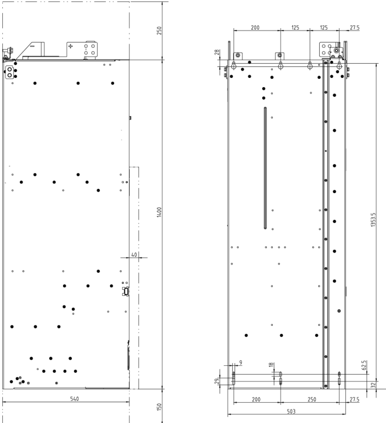
Figure 3-29 Dimension drawing Active Line Module, frame size HX Side view, rear view
