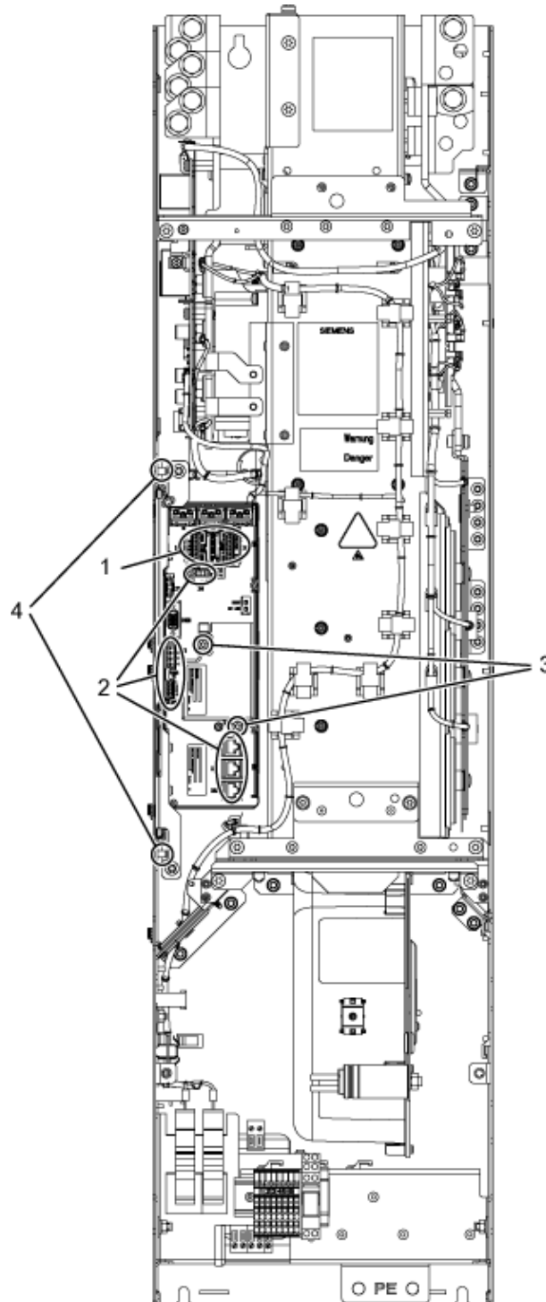
Figure 8-16 Replacing the Control Interface Module, Basic Line Module, frame size FB
