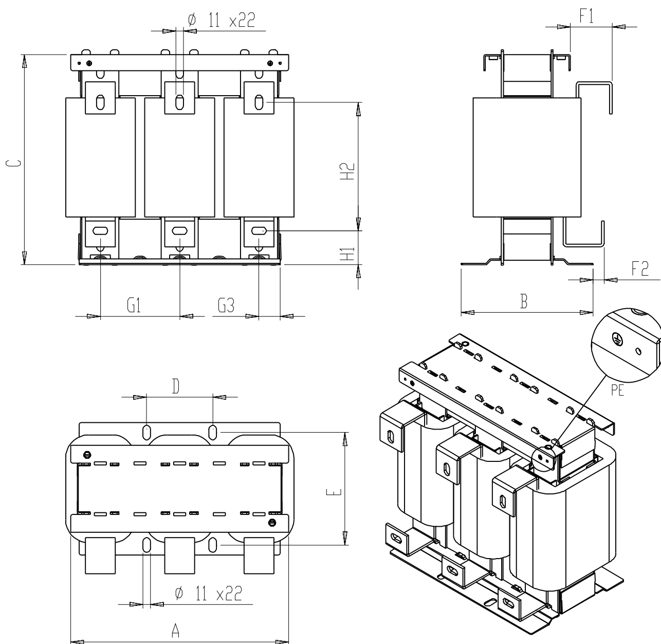
Figure 2-6 Dimension drawing of line reactor 6SL3000-0EH34-7AA0
