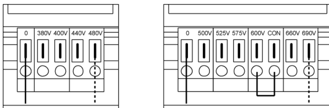
Figure 3-18 Setting terminals for the fan transformers (380 V – 480 V 3 AC / 500 V – 690 V 3 AC)
