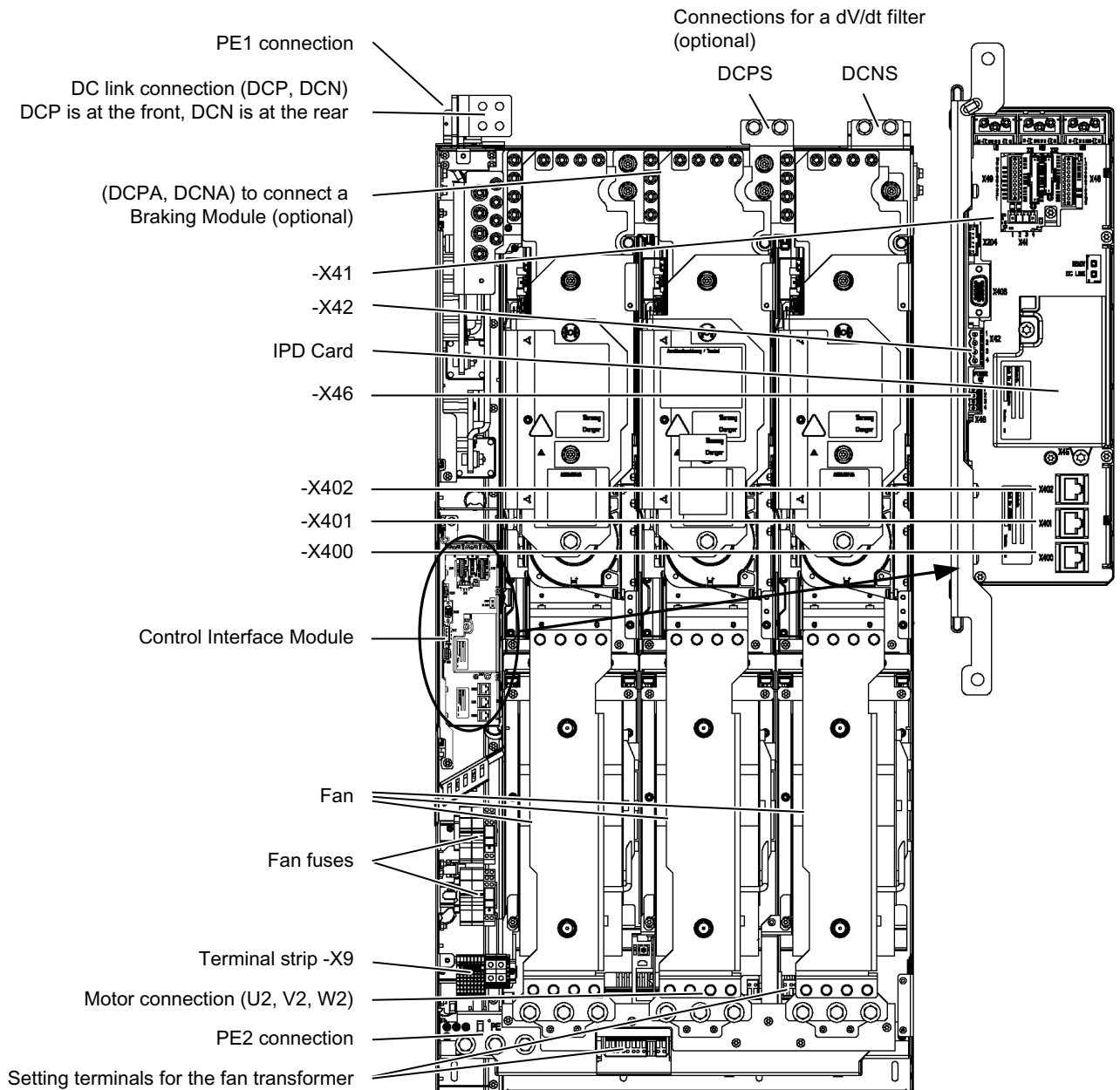
Figure 4-4 Motor Module, frame size JX
