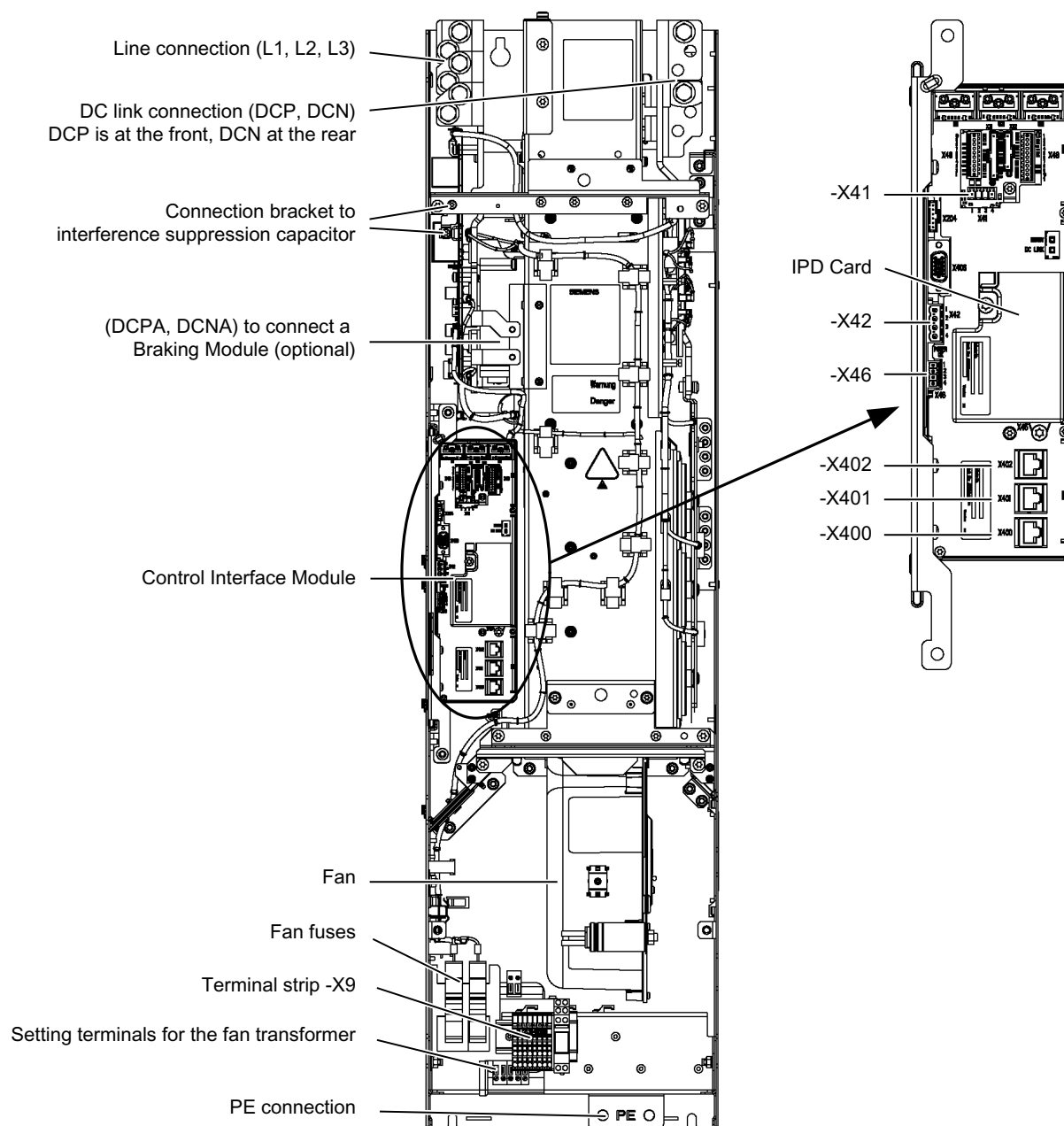
Figure 3-1 Basic Line Module, frame size FB
