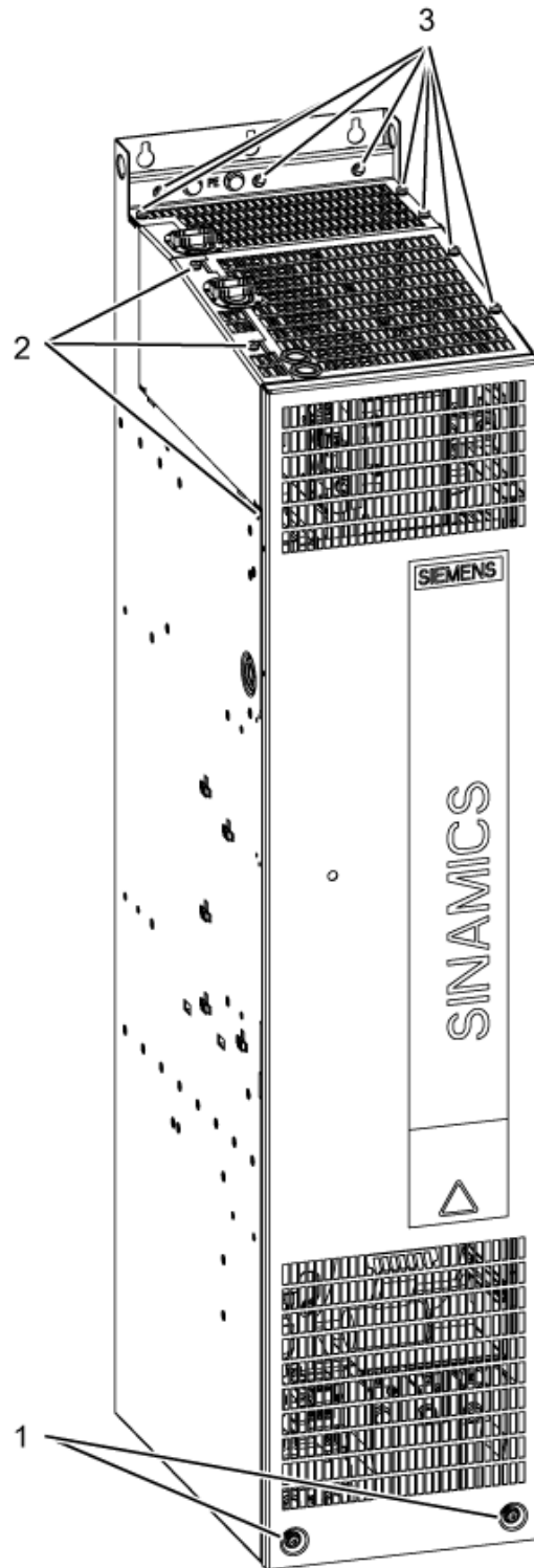
Figure 5-8 Installing the Braking Module in a Smart Line Module / Active Line Module / Motor Module, frame size GX – steps 1 - 3
