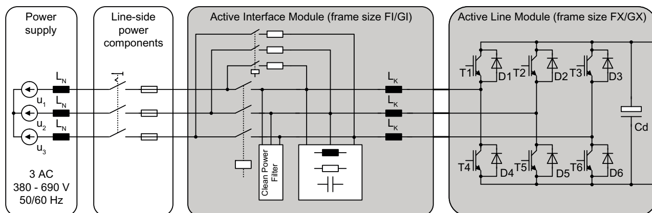
Figure 3-20 Overview of Active Infeed (frame sizes FI/FX and GI/GX)
