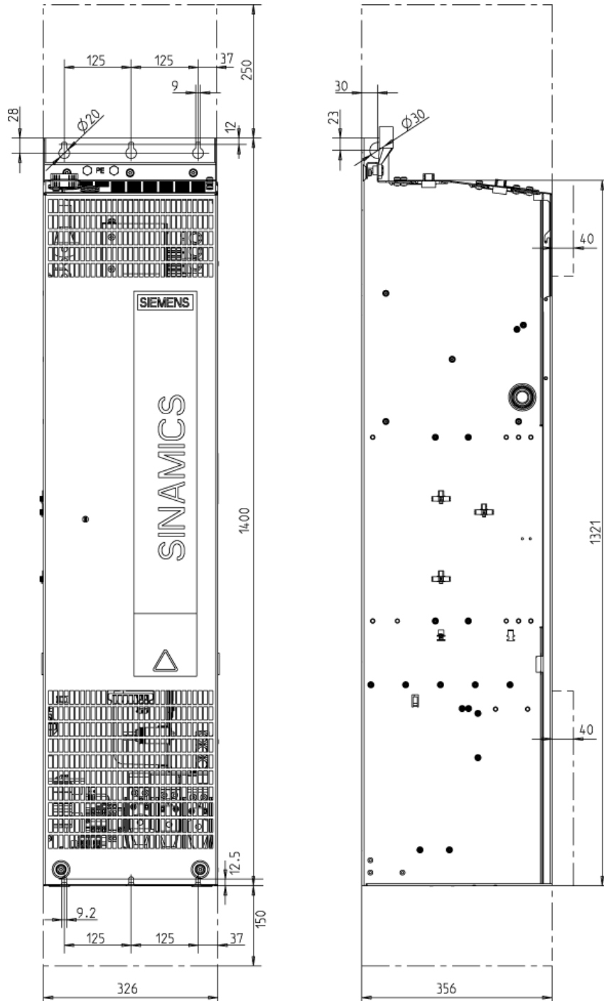
Figure 3-27 Dimension drawing Active Line Module, frame size FX Front view, side view
