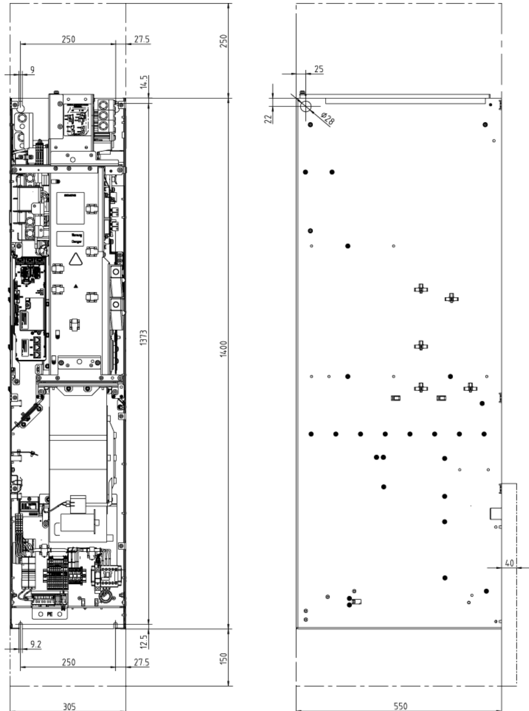
Figure 3-14 Dimension drawing Smart Line Module, frame size GX Front view, side view
