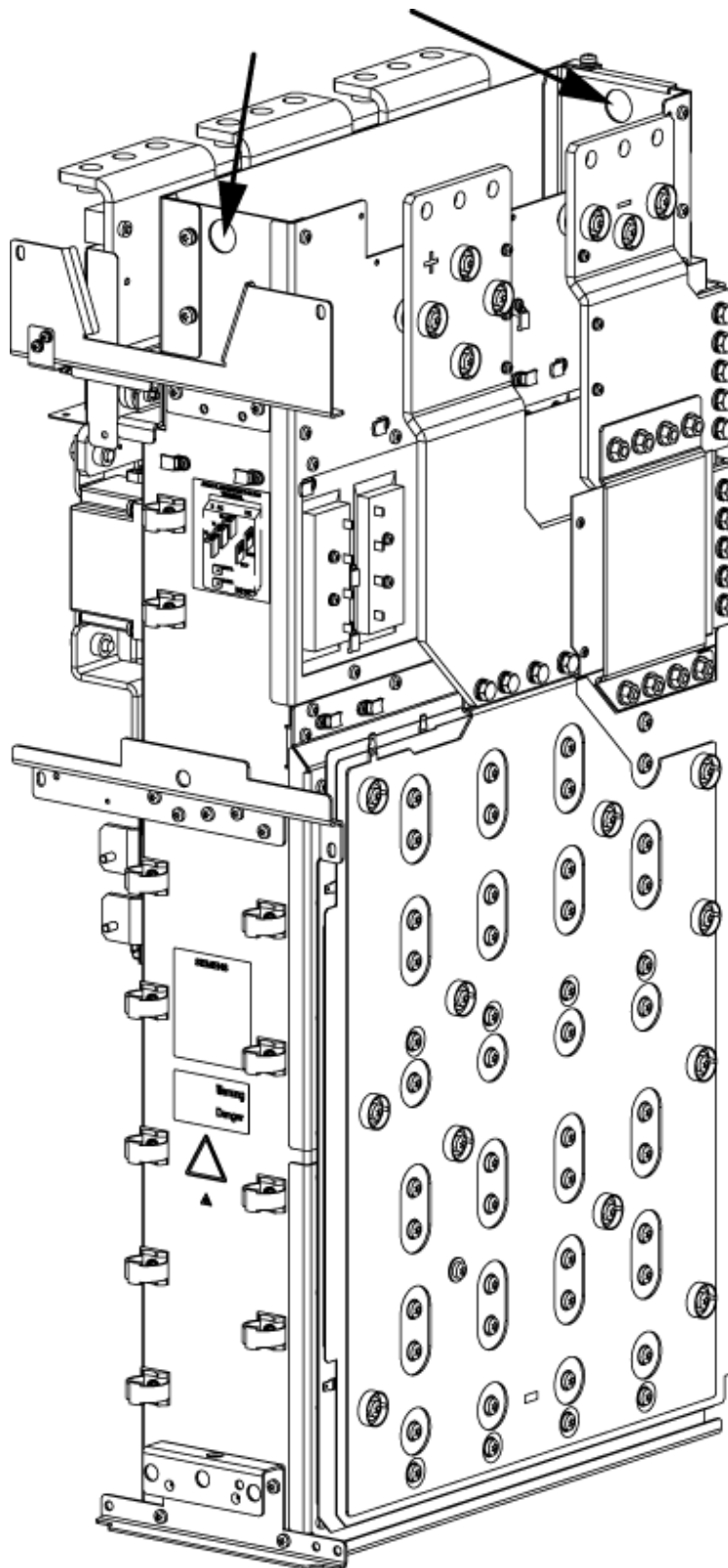
Figure 8-4 Crane lifting lugs on power block frame size GB
