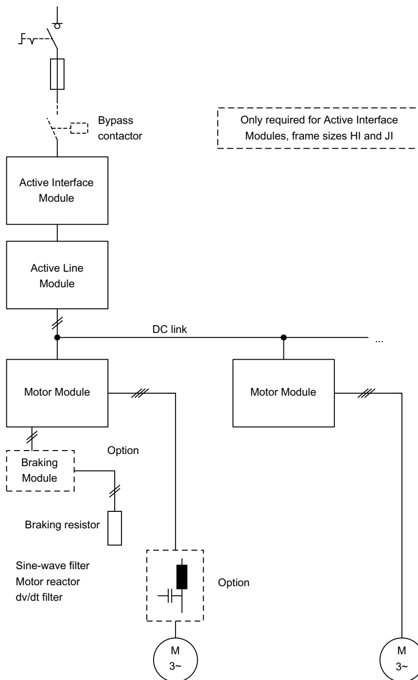
Figure 1-4 Basic structure of a drive system with SINAMICS S120 and regulated infeed
