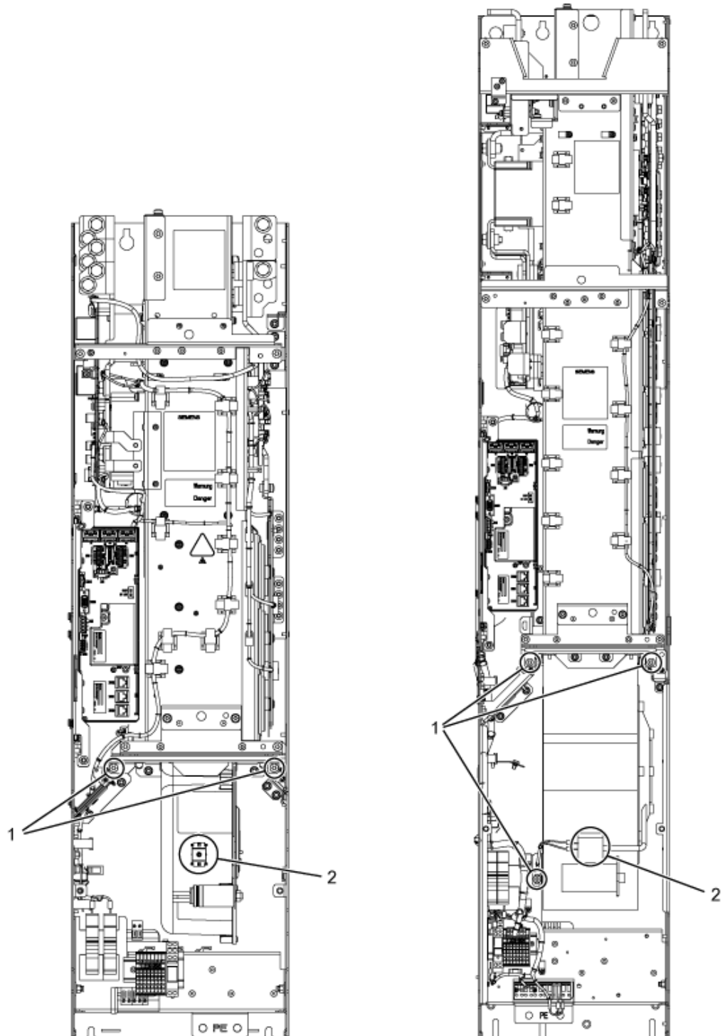
Figure 8-26 Replacing the fan, Basic Line Module, frame sizes FB, GB
