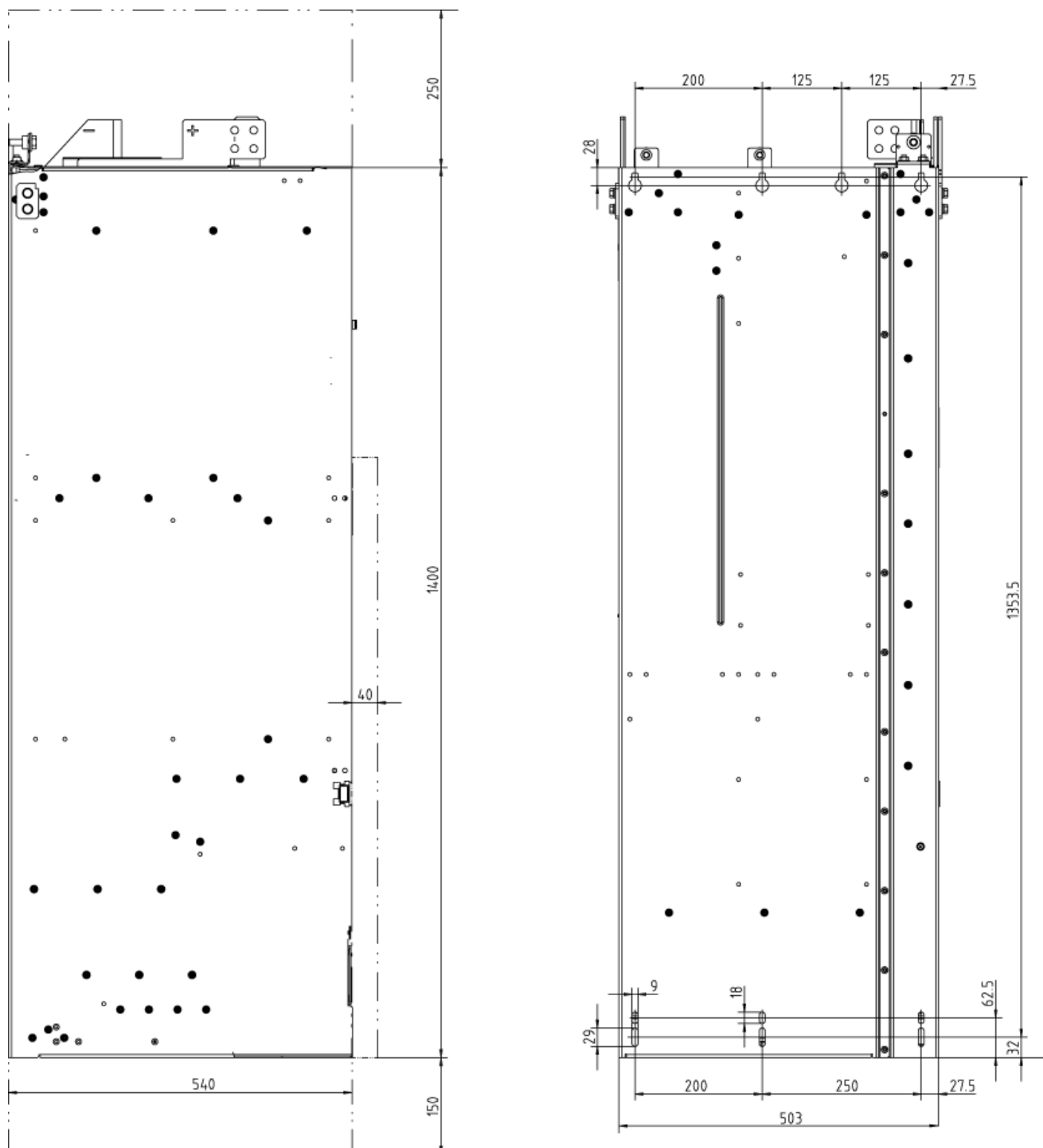
Figure 3-15 Dimension drawing Smart Line Module, frame size HX Side view, rear view
