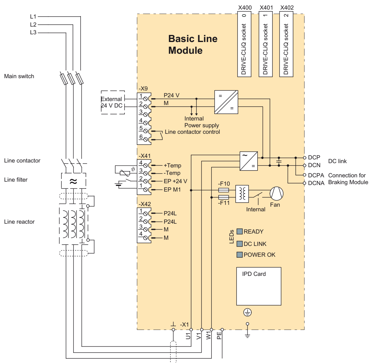
Figure 3-3 Connection example for Basic Line Modules
