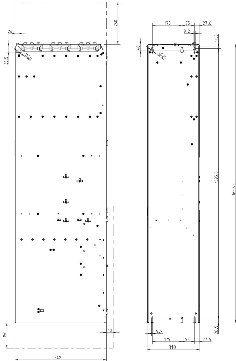
Figure 3-5 Dimension drawing, Basic Line Module, frame size GB Side view, rear view
