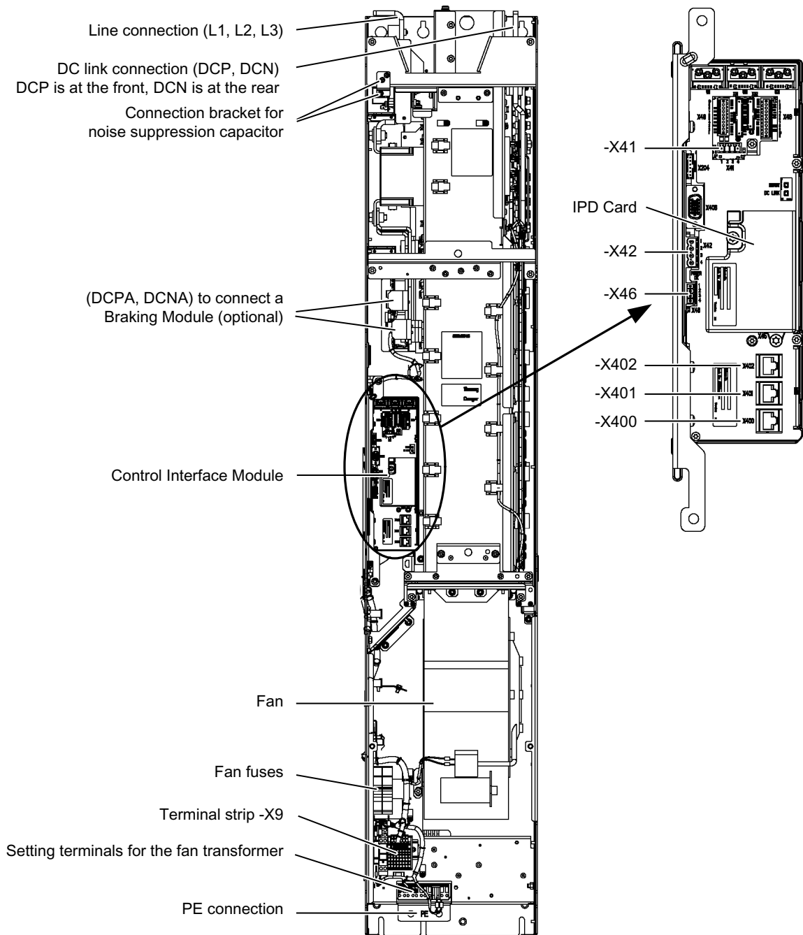
Figure 3-2 Basic Line Module, frame size GB
