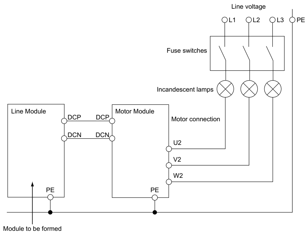
Figure 8-28 Forming circuit for Line Modules
