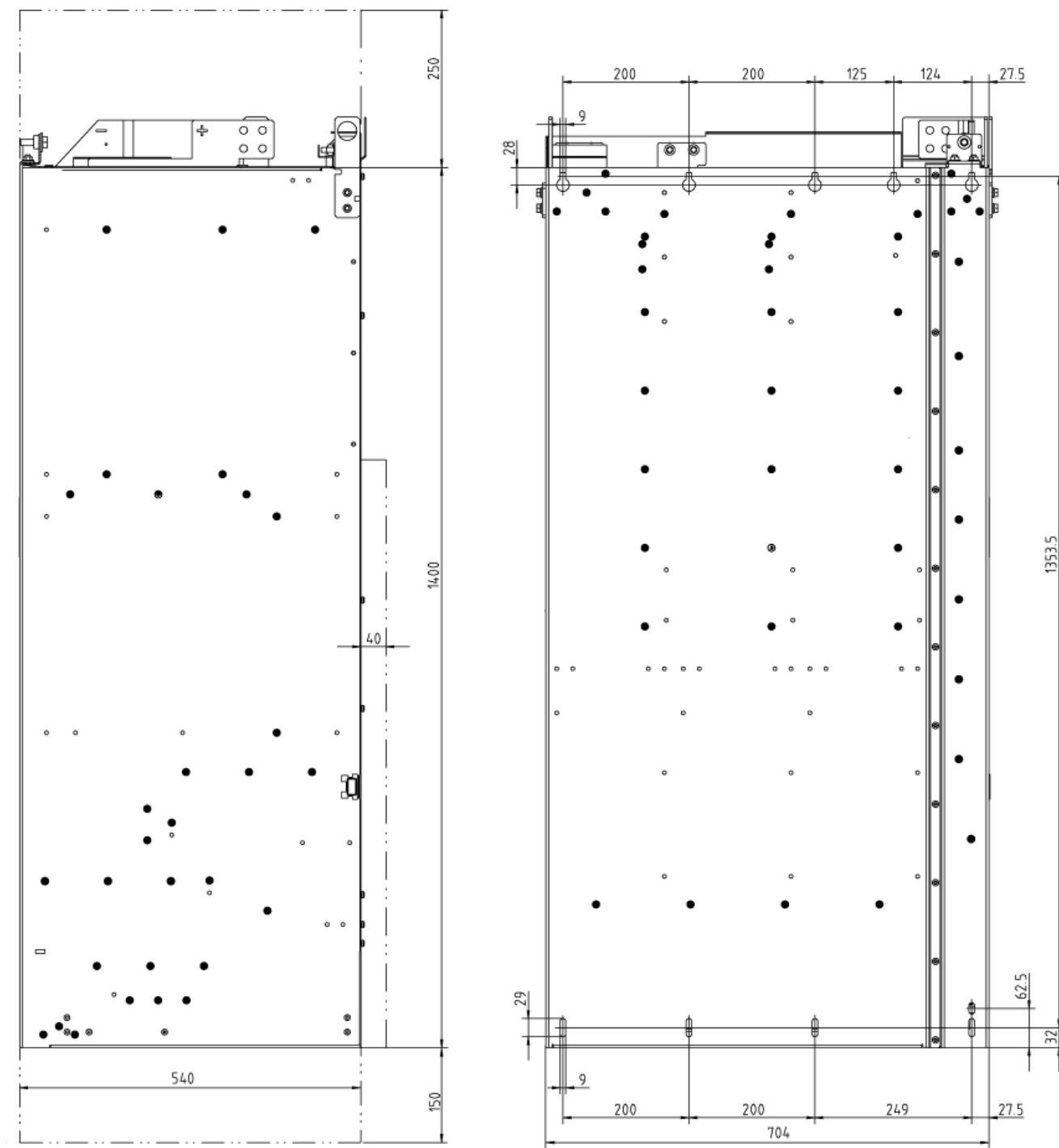
Figure 3-30 Dimension drawing Active Line Module, frame size JX Side view, rear view
