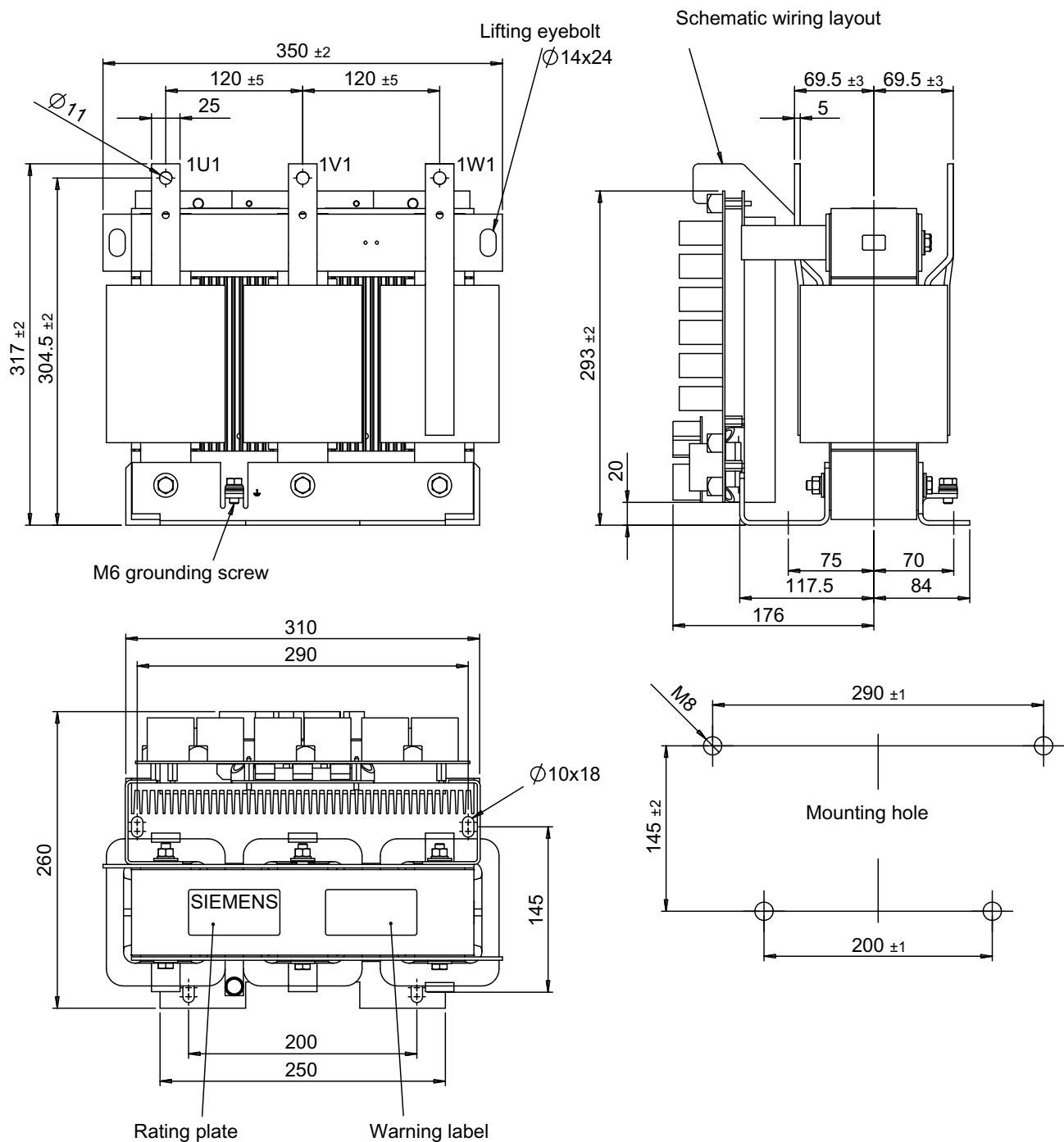
Figure 6-21 Dimension drawing for dv/dt filter compact plus Voltage Peak Limiter, Type 2
