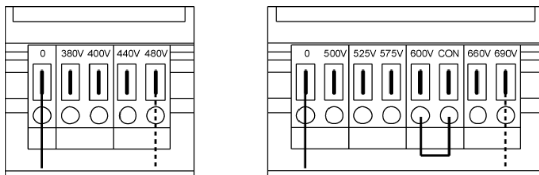
Figure 3-7 Setting terminals for the fan transformers (380 V – 480 V 3 AC / 500 V – 690 V 3 AC)
