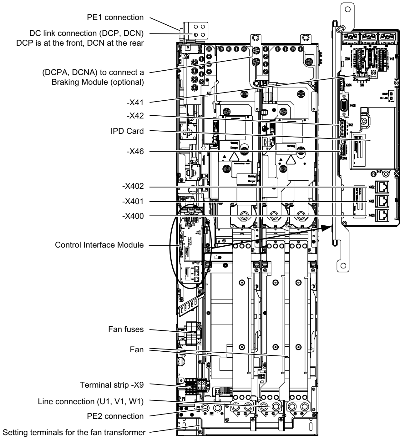
Figure 3-24 Active Line Module, frame size HX
